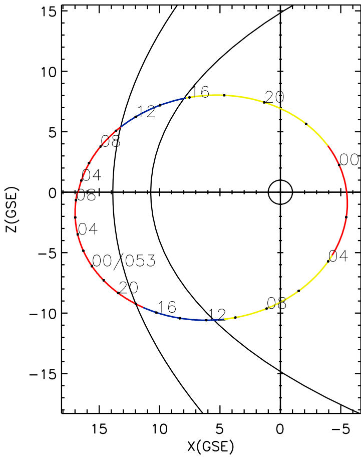
CLUSTER 2 orbit 2017 051 (02/20) 02:36 UT to 2017 053 (02/22) 08:51 UT
