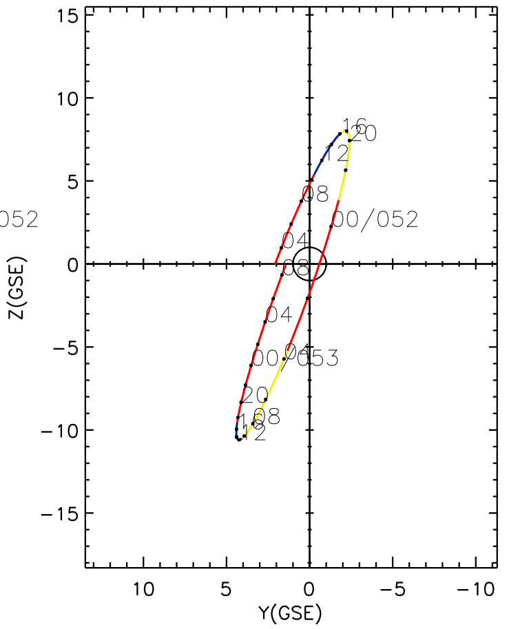
CLUSTER 2 orbit 2017 051 (02/20) 02:36 UT to 2017 053 (02/22) 08:51 UT
