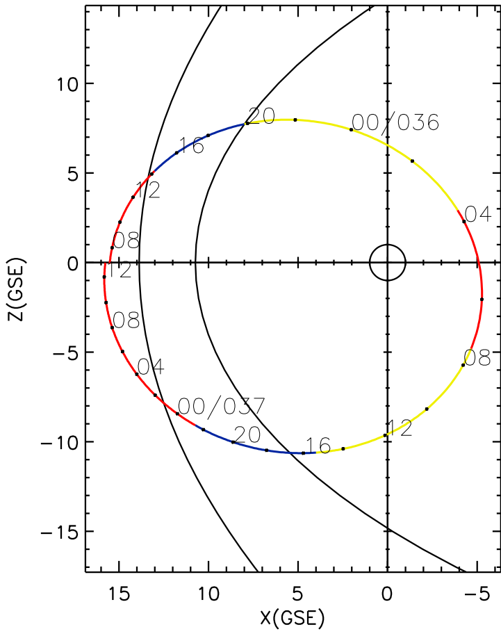
CLUSTER 2 orbit 2017 035 (02/04) 06:46 UT to 2017 037 (02/06) 13:06 UT
