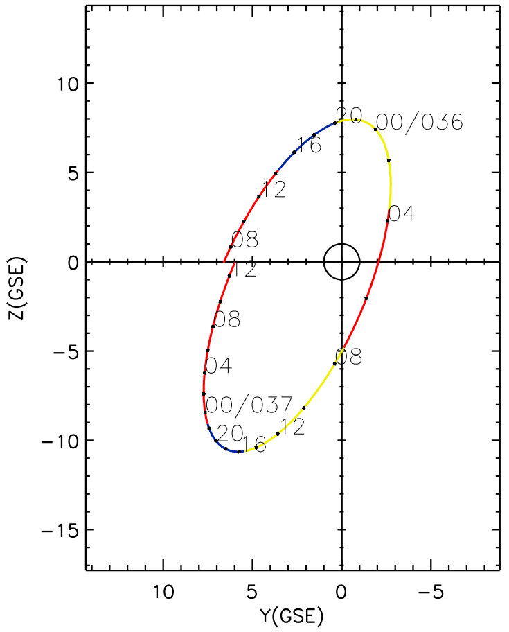
CLUSTER 2 orbit 2017 035 (02/04) 06:46 UT to 2017 037 (02/06) 13:06 UT
