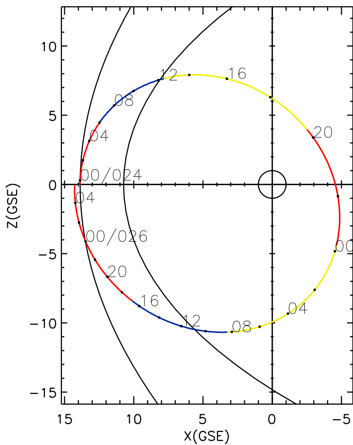
CLUSTER 2 orbit 2017 023 (01/23) 23:31 UT to 2017 026 (01/26) 05:46 UT
