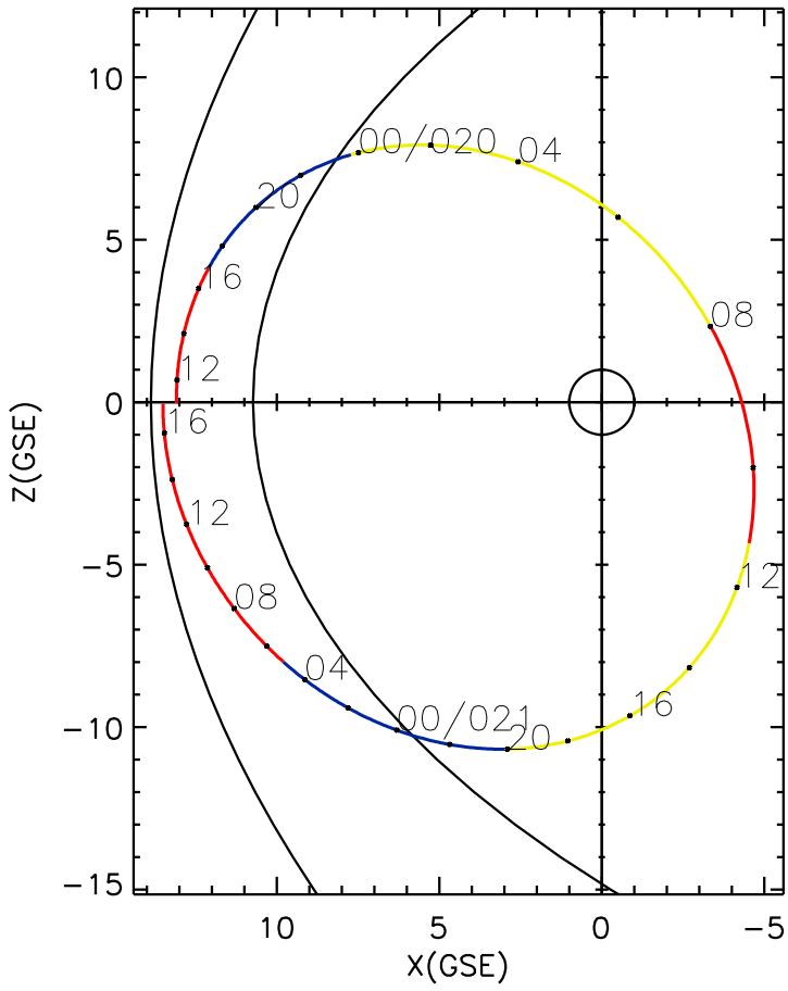
CLUSTER 2 orbit 2017 019 (01/19) 11:01 UT to 2017 021 (01/21) 17:16 UT
