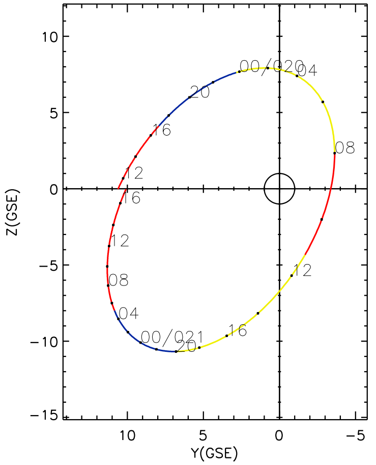
CLUSTER 2 orbit 2017 019 (01/19) 11:01 UT to 2017 021 (01/21) 17:16 UT
