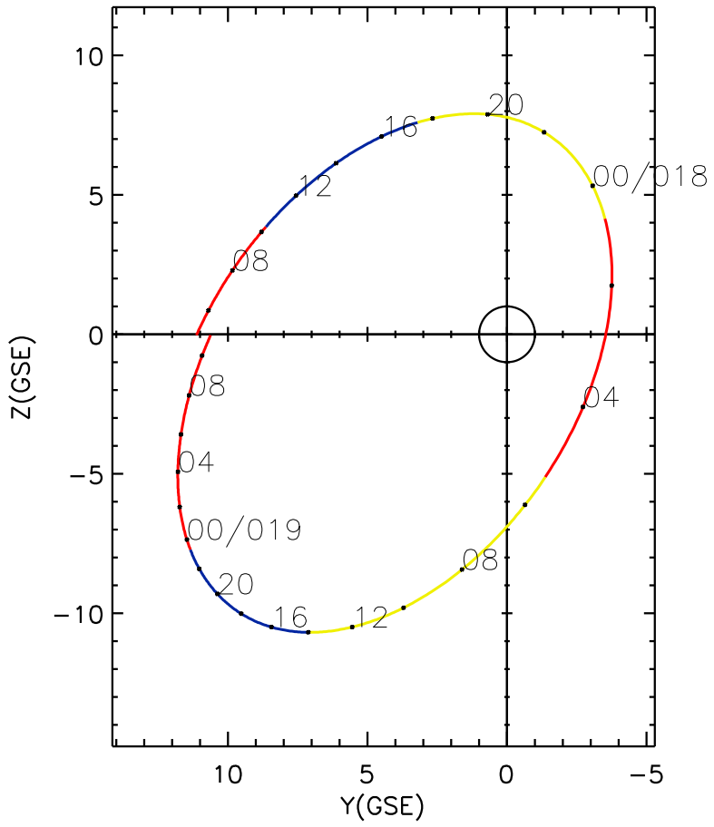
CLUSTER 2 orbit 2017 017 (01/17) 04:46 UT to 2017 019 (01/19) 11:01 UT
