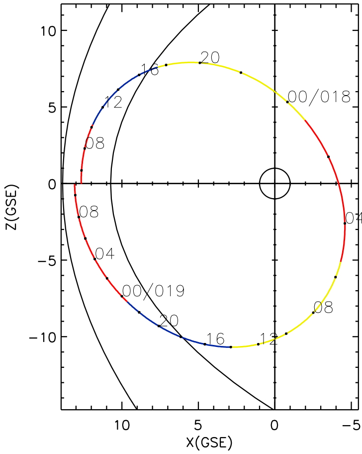
CLUSTER 2 orbit 2017 017 (01/17) 04:46 UT to 2017 019 (01/19) 11:01 UT
