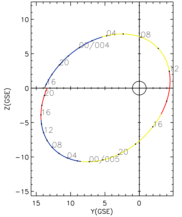
CLUSTER 2 orbit 2017 003 (01/03) 15:11 UT to 2017 005 (01/05) 21:26 UT
