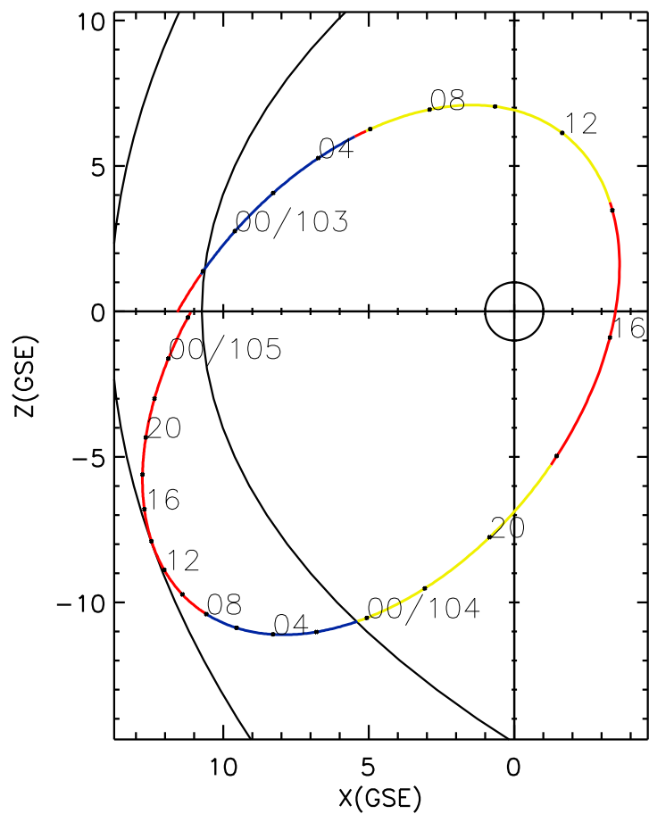
CLUSTER 2 orbit 2016 102 (04/11) 20:01 UT to 2016 105 (04/14) 02:16 UT
