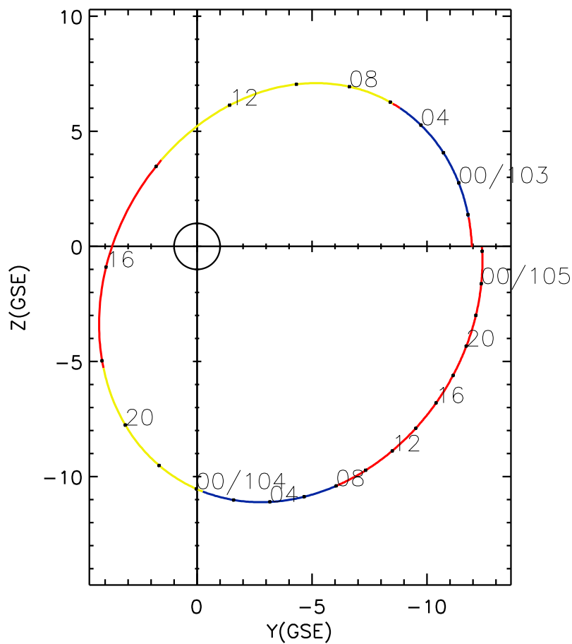
CLUSTER 2 orbit 2016 102 (04/11) 20:01 UT to 2016 105 (04/14) 02:16 UT
