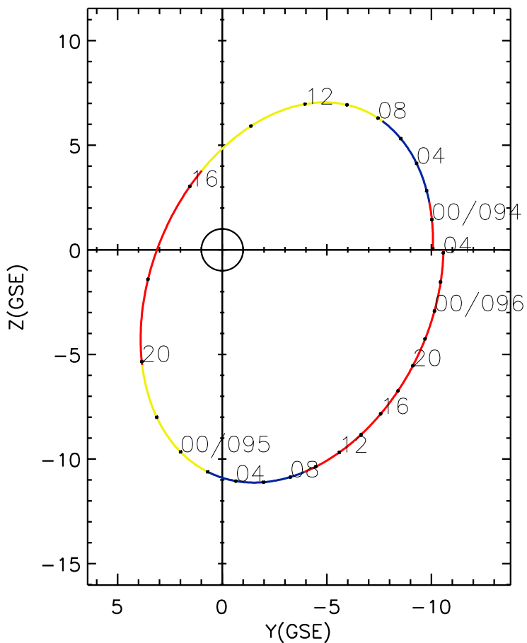
CLUSTER 2 orbit 2016 093 (04/02) 21:51 UT to 2016 096 (04/05) 04:11 UT
