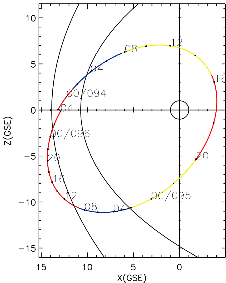
CLUSTER 2 orbit 2016 093 (04/02) 21:51 UT to 2016 096 (04/05) 04:11 UT
