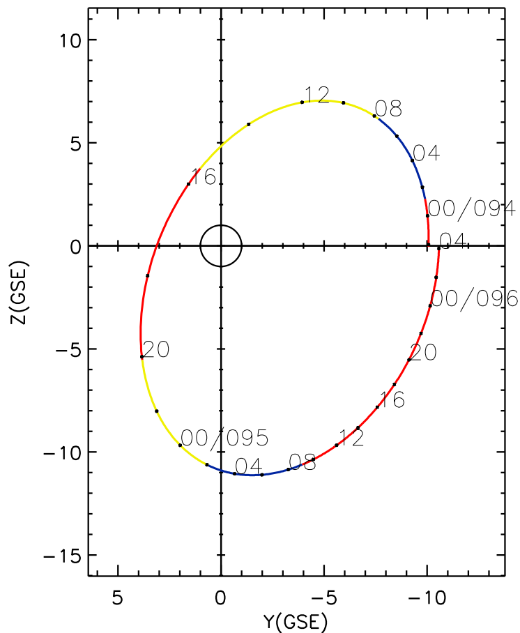
CLUSTER 2 orbit 2016 093 (04/02) 21:51 UT to 2016 096 (04/05) 04:06 UT
