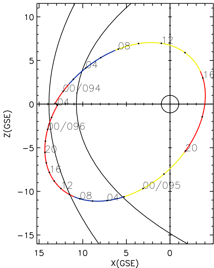
CLUSTER 2 orbit 2016 093 (04/02) 21:51 UT to 2016 096 (04/05) 04:06 UT
