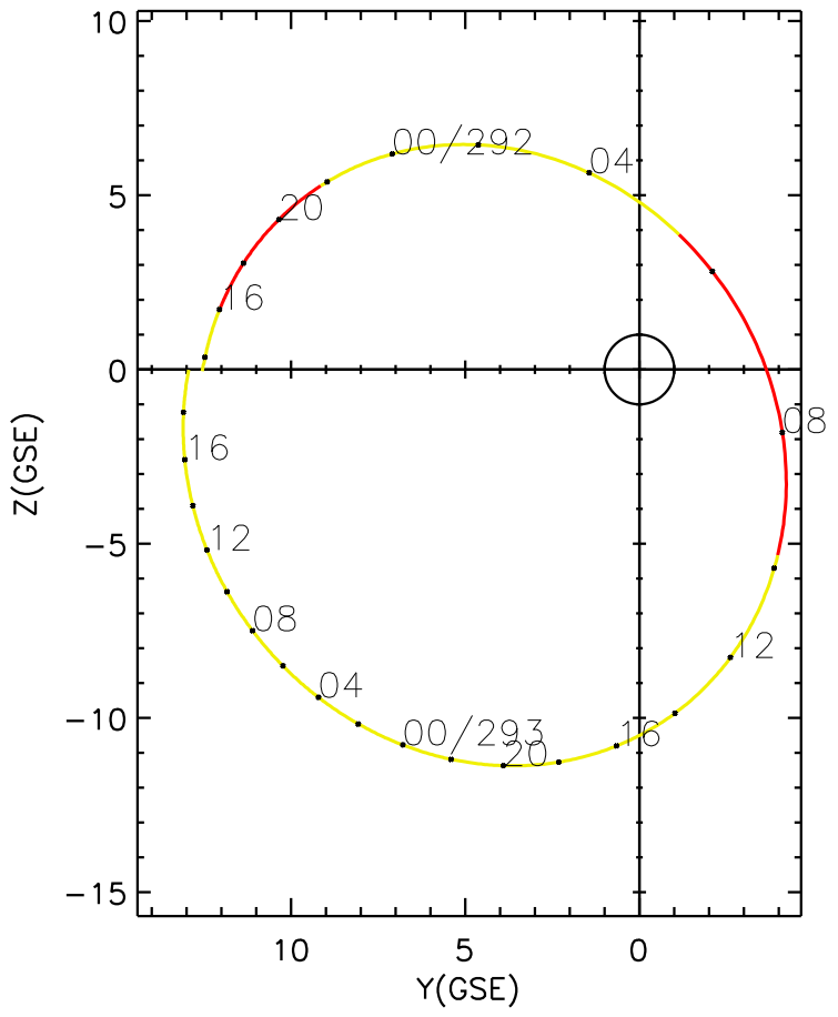
CLUSTER 2 orbit 2015 291 (10/18) 13:26 UT to 2015 293 (10/20) 19:46 UT
