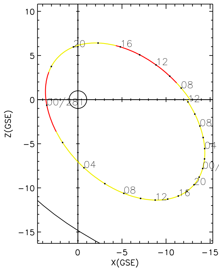
CLUSTER 2 orbit 2015 280 (10/07) 06:06 UT to 2015 282 (10/09) 12:21 UT
