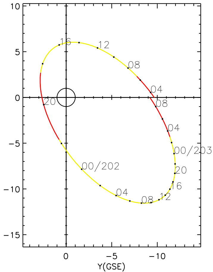
CLUSTER 2 orbit 2015 201 (07/20) 03:11 UT to 2015 203 (07/22) 09:26 UT
