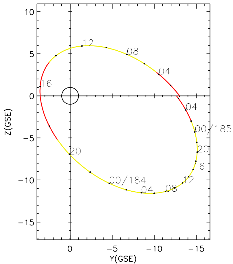
CLUSTER 2 orbit 2015 183 (07/02) 00:11 UT to 2015 185 (07/04) 06:26 UT
