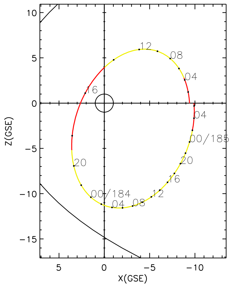
CLUSTER 2 orbit 2015 183 (07/02) 00:11 UT to 2015 185 (07/04) 06:26 UT
