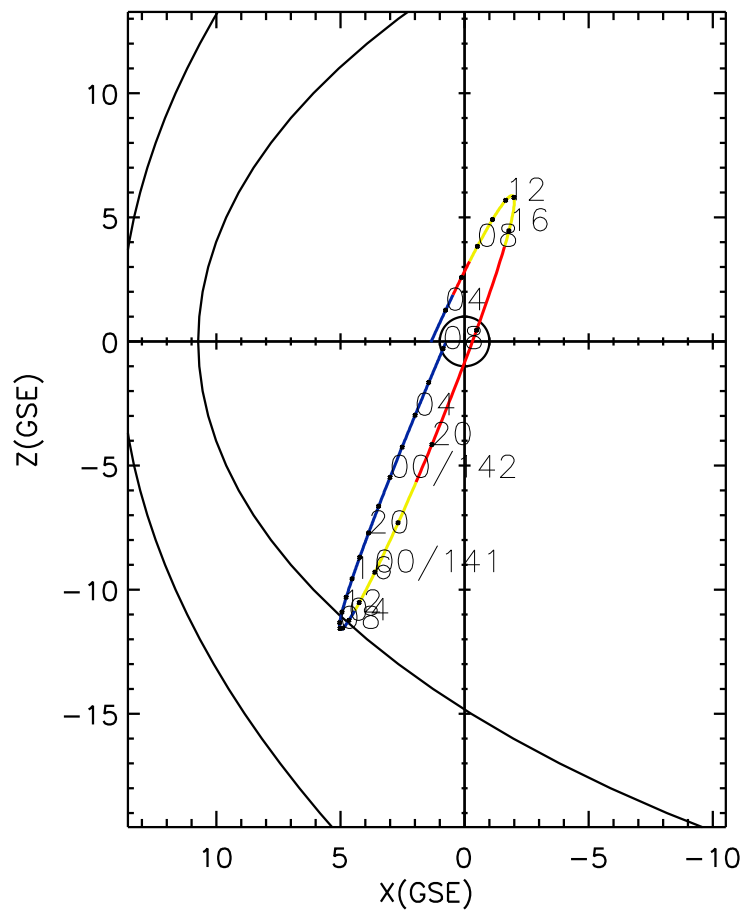
CLUSTER 2 orbit 2015 140 (05/20) 02:06 UT to 2015 142 (05/22) 08:21 UT
