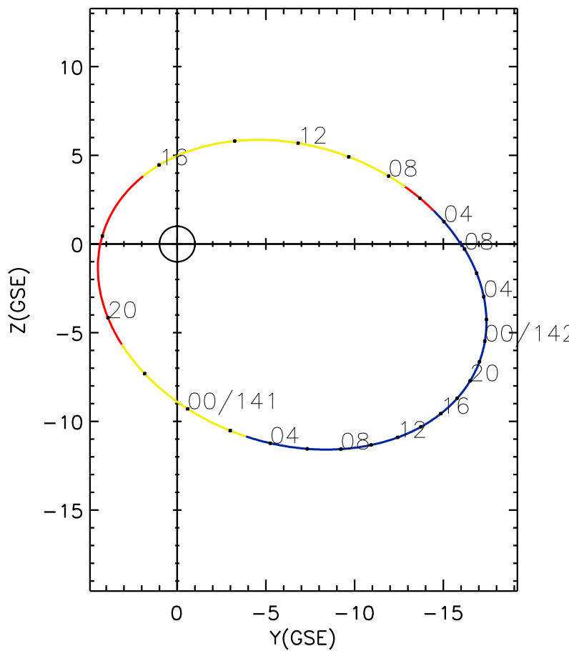
CLUSTER 2 orbit 2015 140 (05/20) 02:06 UT to 2015 142 (05/22) 08:21 UT
