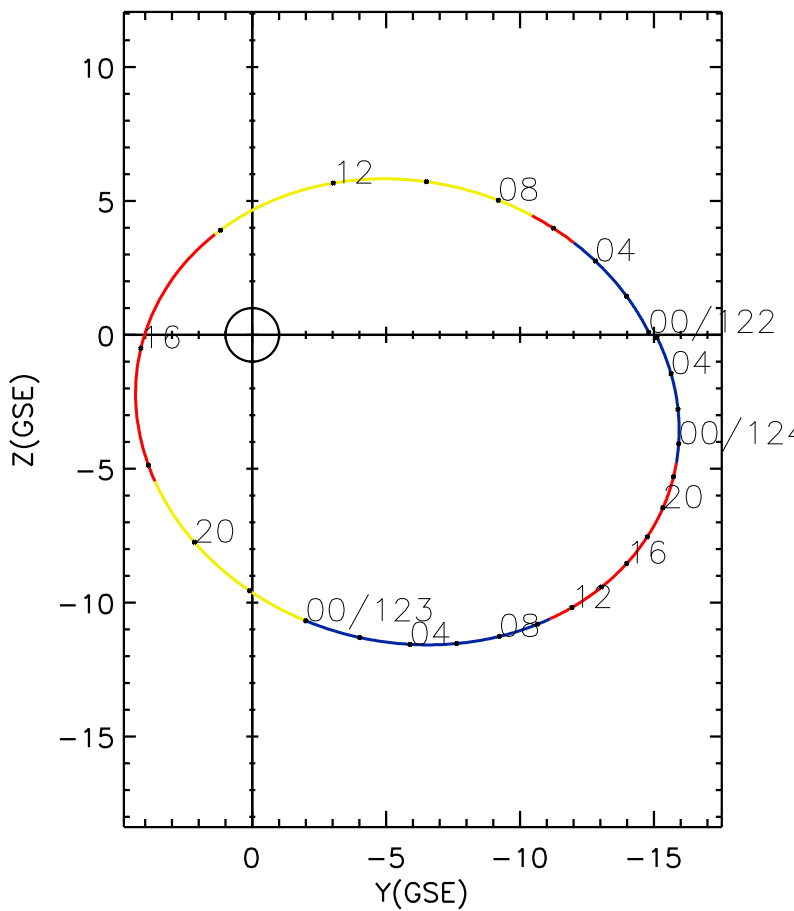
CLUSTER 2 orbit 2015 121 (05/01) 23:51 UT to 2015 124 (05/04) 06:06 UT
