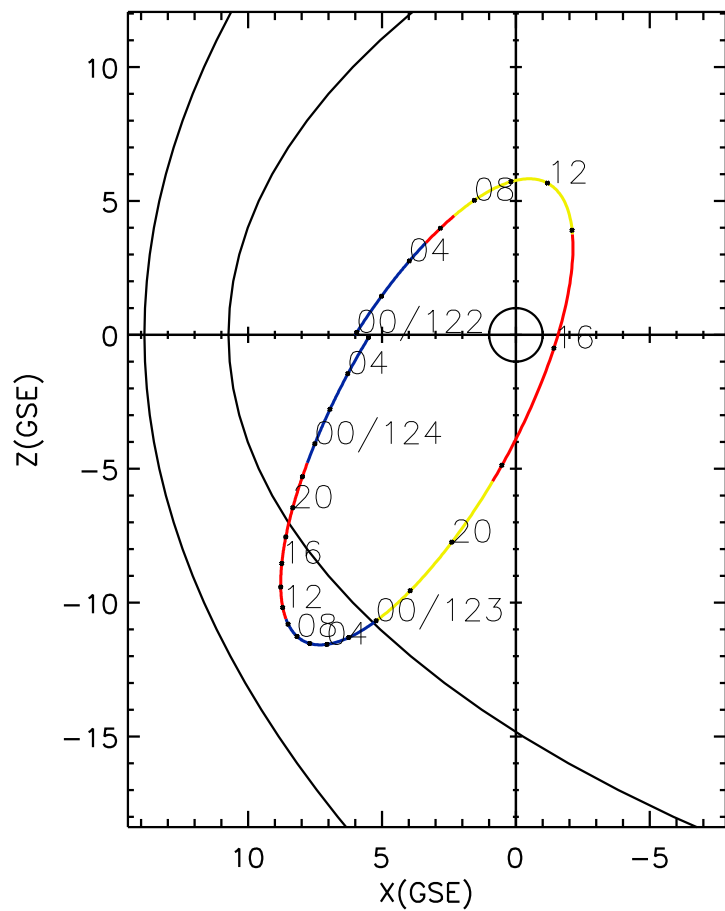
CLUSTER 2 orbit 2015 121 (05/01) 23:51 UT to 2015 124 (05/04) 06:06 UT
