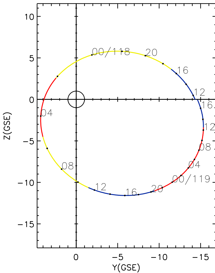
CLUSTER 2 orbit 2015 117 (04/27) 11:16 UT to 2015 119 (04/29) 17:31 UT
