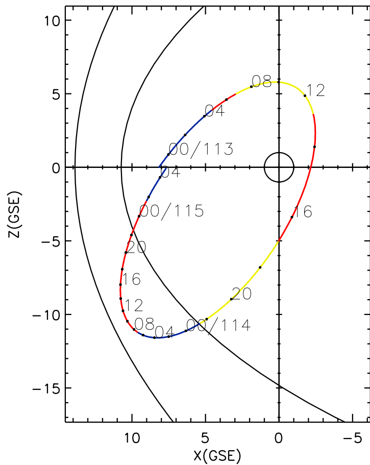
CLUSTER 2 orbit 2015 112 (04/22) 22:41 UT to 2015 115 (04/25) 04:56 UT
