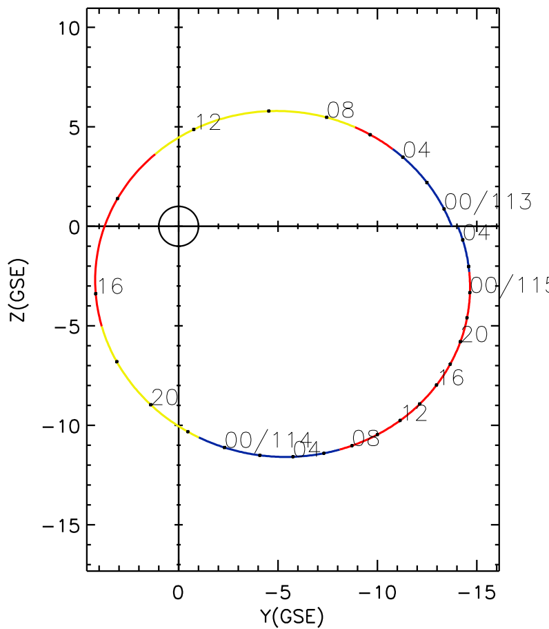
CLUSTER 2 orbit 2015 112 (04/22) 22:41 UT to 2015 115 (04/25) 04:56 UT
