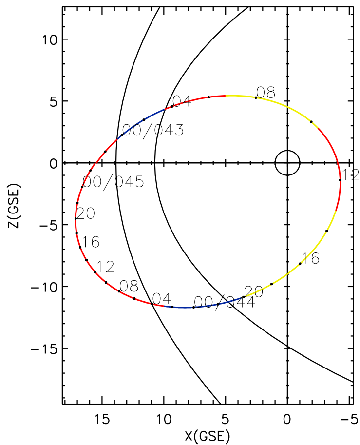
CLUSTER 2 orbit 2015 042 (02/11) 20:36 UT to 2015 045 (02/14) 02:51 UT
