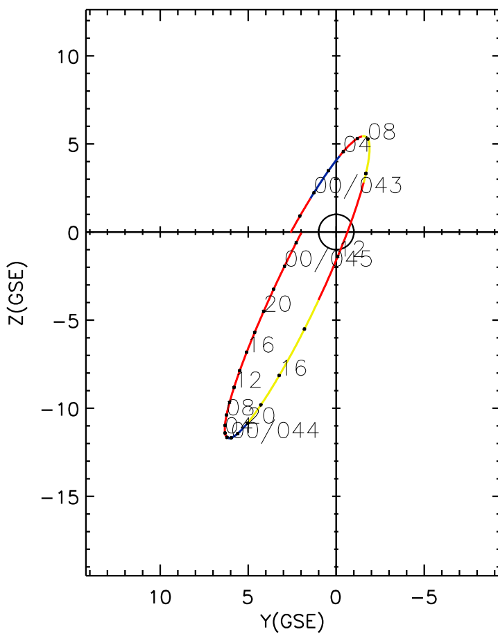
CLUSTER 2 orbit 2015 042 (02/11) 20:36 UT to 2015 045 (02/14) 02:51 UT
