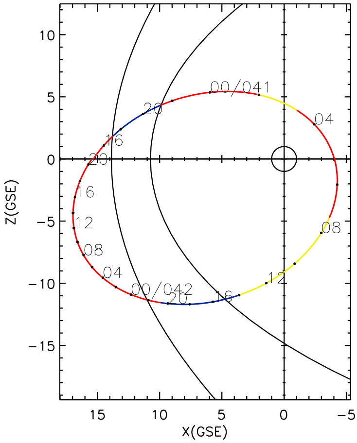
CLUSTER 2 orbit 2015 040 (02/09) 14:21 UT to 2015 042 (02/11) 20:36 UT
