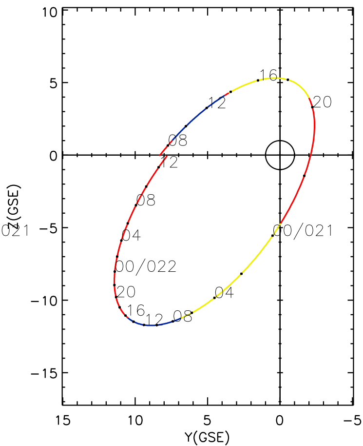
CLUSTER 2 orbit 2015 020 (01/20) 06:56 UT to 2015 022 (01/22) 13:11 UT
