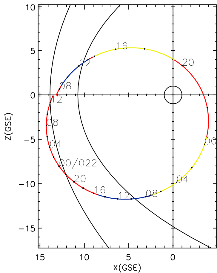
CLUSTER 2 orbit 2015 020 (01/20) 06:56 UT to 2015 022 (01/22) 13:11 UT
