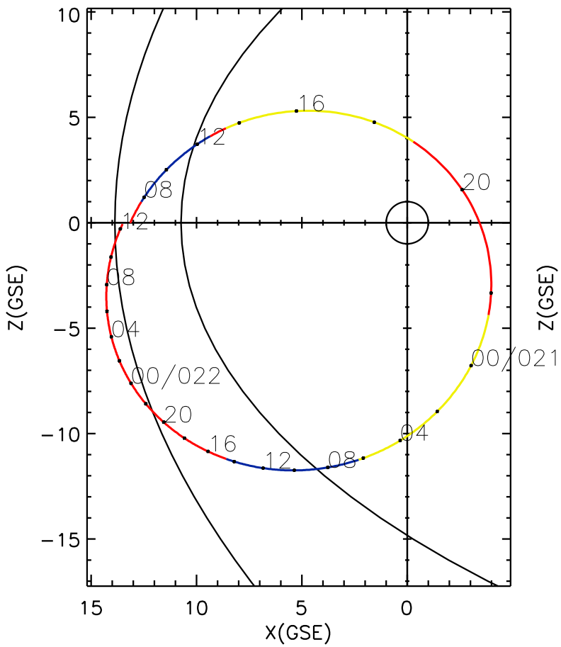
CLUSTER 2 orbit 2015 020 (01/20) 06:11 UT to 2015 022 (01/22) 12:21 UT
