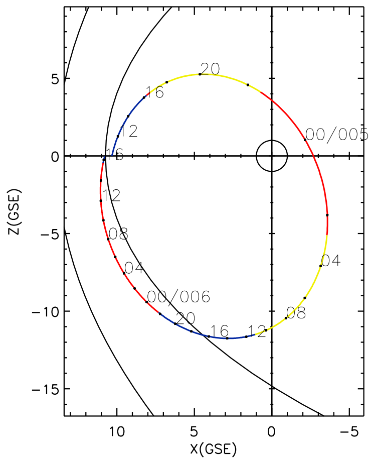
CLUSTER 2 orbit 2015 004 (01/04) 10:06 UT to 2015 006 (01/06) 16:21 UT
