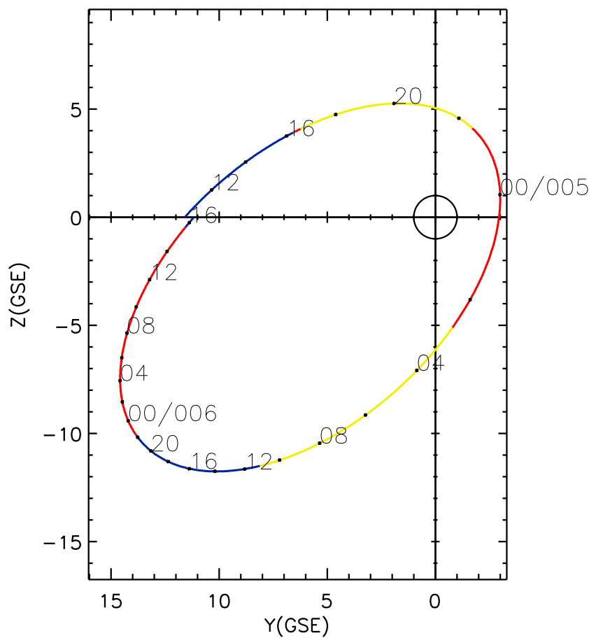
CLUSTER 2 orbit 2015 004 (01/04) 10:06 UT to 2015 006 (01/06) 16:21 UT
