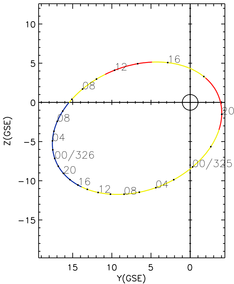
CLUSTER 2 orbit 2014 324 (11/20) 05:21 UT to 2014 326 (11/22) 11:36 UT
