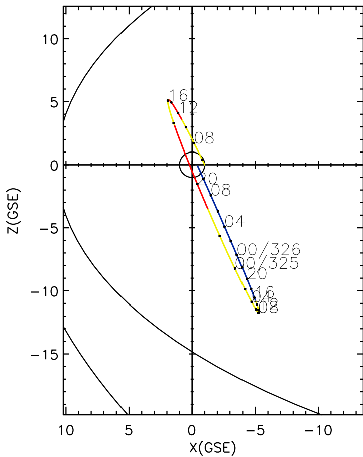
CLUSTER 2 orbit 2014 324 (11/20) 05:21 UT to 2014 326 (11/22) 11:36 UT
