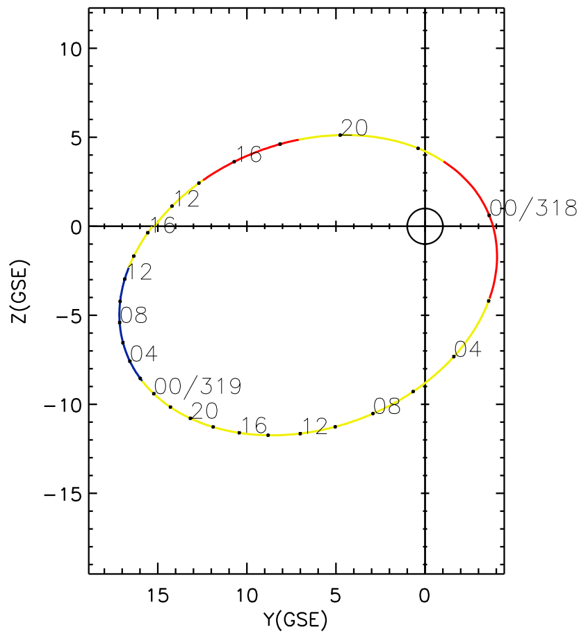
CLUSTER 2 orbit 2014 317 (11/13) 10:16 UT to 2014 319 (11/15) 16:31 UT
