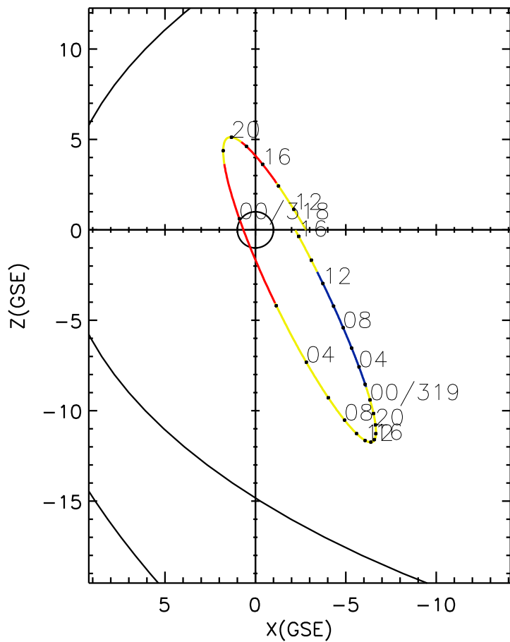
CLUSTER 2 orbit 2014 317 (11/13) 10:16 UT to 2014 319 (11/15) 16:31 UT
