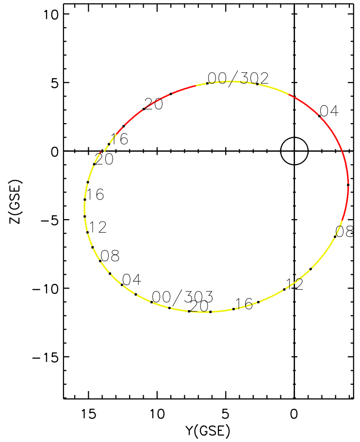
CLUSTER 2 orbit 2014 301 (10/28) 15:11 UT to 2014 303 (10/30) 21:26 UT
