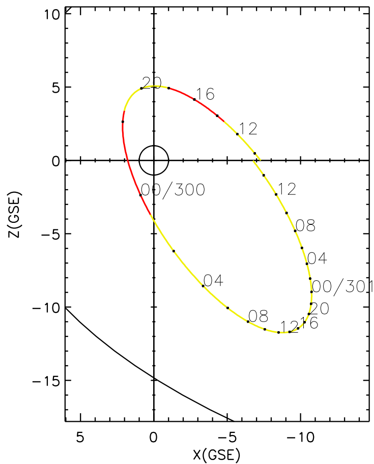
CLUSTER 2 orbit 2014 299 (10/26) 09:16 UT to 2014 301 (10/28) 15:31 UT
