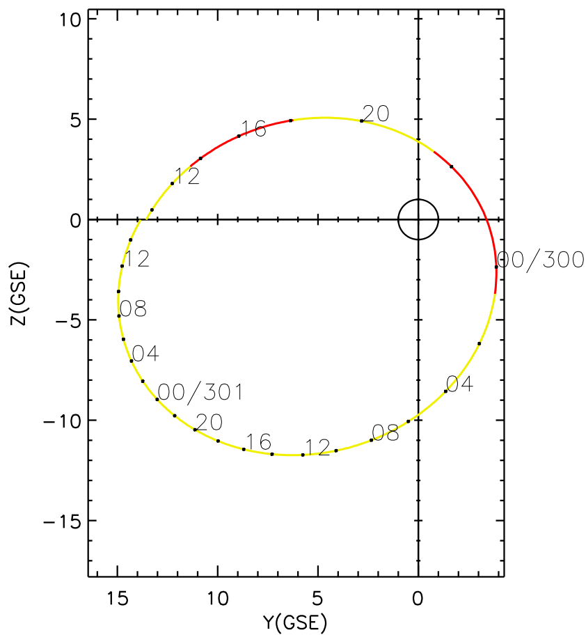
CLUSTER 2 orbit 2014 299 (10/26) 09:16 UT to 2014 301 (10/28) 15:31 UT
