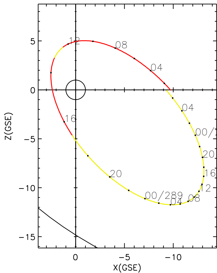
CLUSTER 2 orbit 2014 288 (10/15) 00:56 UT to 2014 290 (10/17) 07:11 UT
