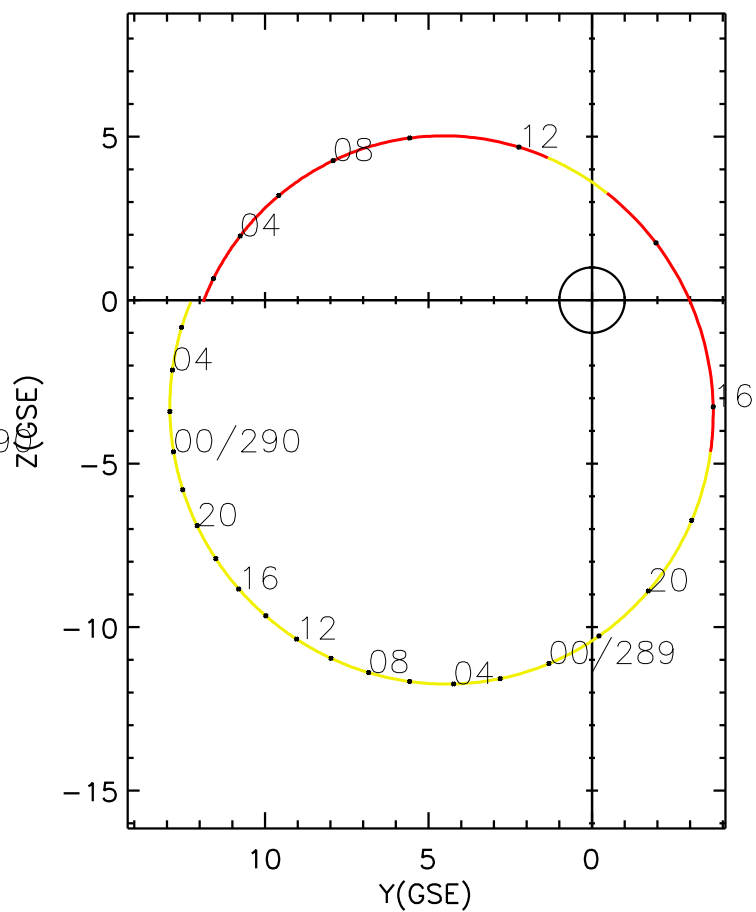
CLUSTER 2 orbit 2014 288 (10/15) 00:56 UT to 2014 290 (10/17) 07:11 UT
