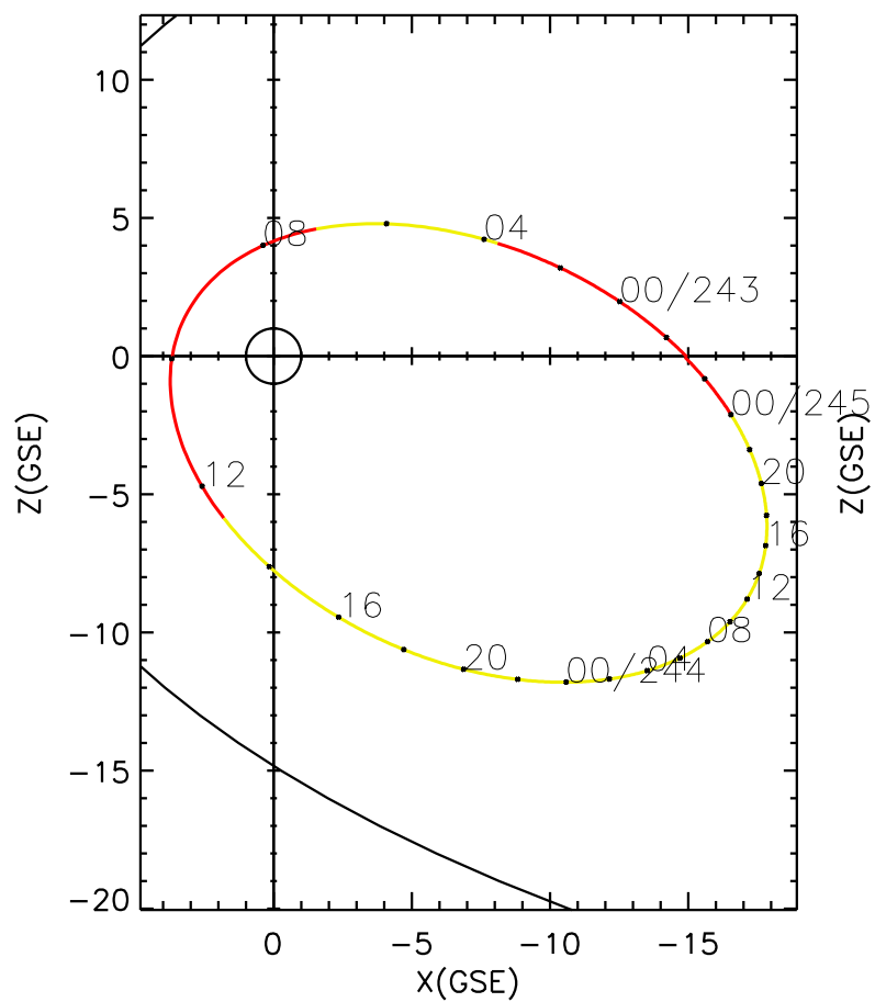
CLUSTER 2 orbit 2014 242 (08/30) 20:56 UT to 2014 245 (09/02) 03:11 UT
