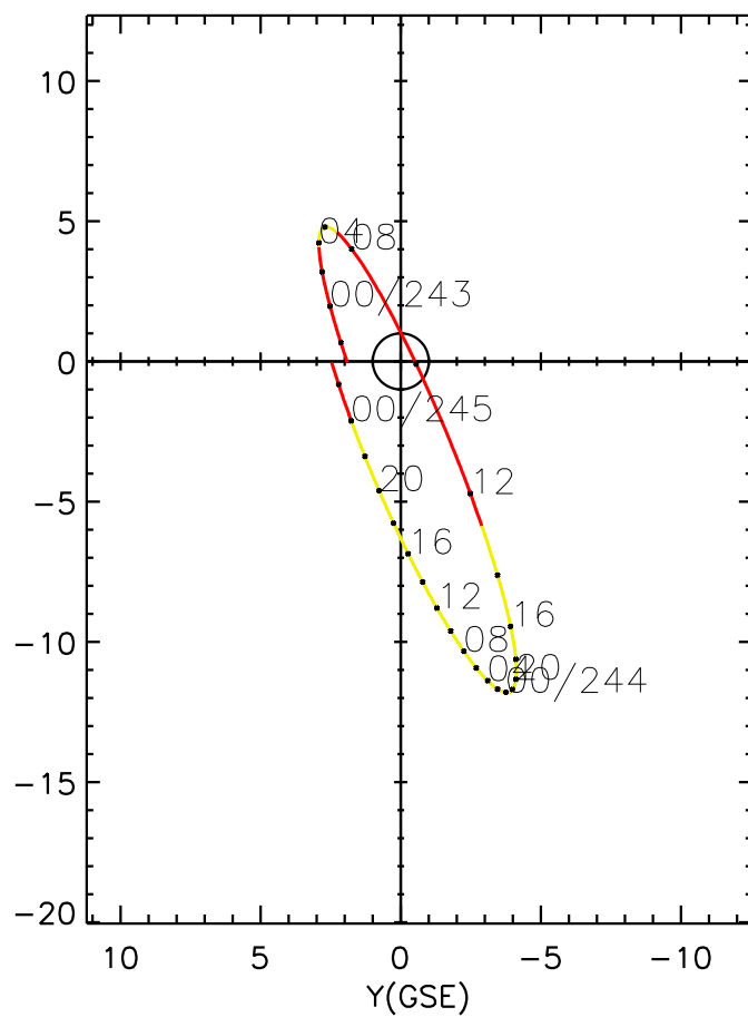
CLUSTER 2 orbit 2014 242 (08/30) 20:56 UT to 2014 245 (09/02) 03:11 UT
