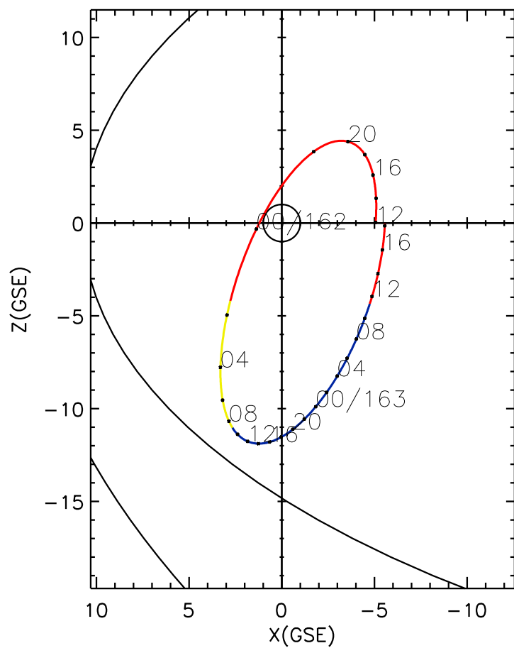
CLUSTER 2 orbit 2014 161 (06/10) 11:56 UT to 2014 163 (06/12) 18:11 UT
