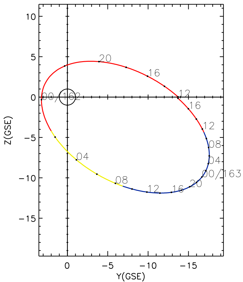
CLUSTER 2 orbit 2014 161 (06/10) 11:56 UT to 2014 163 (06/12) 18:11 UT
