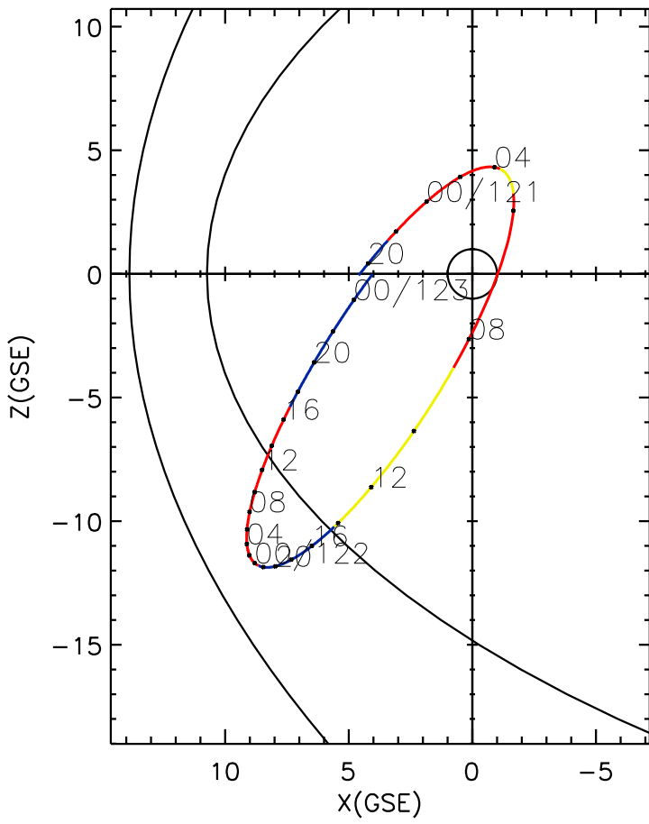
CLUSTER 2 orbit 2014 120 (04/30) 19:16 UT to 2014 123 (05/03) 01:36 UT
