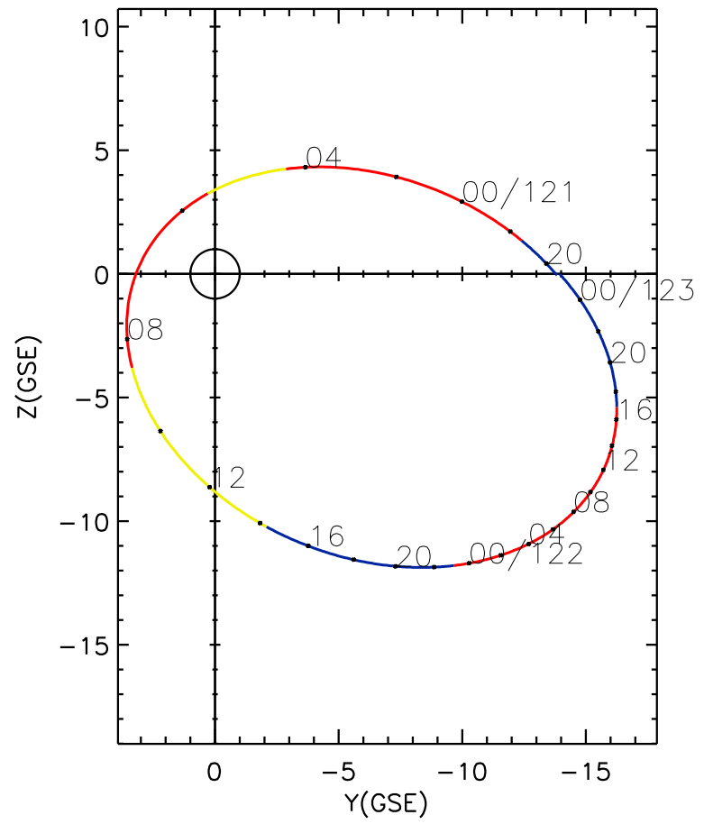
CLUSTER 2 orbit 2014 120 (04/30) 19:16 UT to 2014 123 (05/03) 01:36 UT
