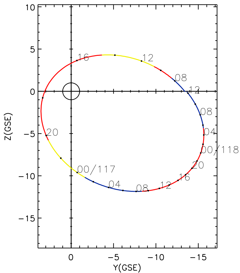
CLUSTER 2 orbit 2014 116 (04/26) 06:01 UT to 2014 118 (04/28) 12:16 UT
