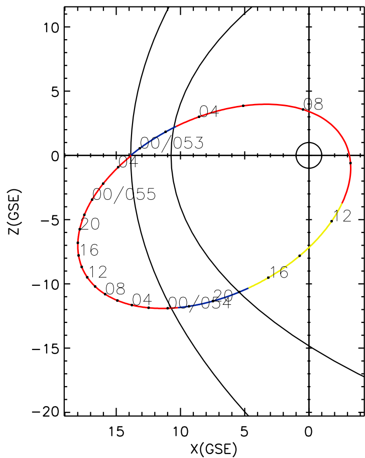
CLUSTER 2 orbit 2014 052 (02/21) 23:06 UT to 2014 055 (02/24) 05:21 UT
