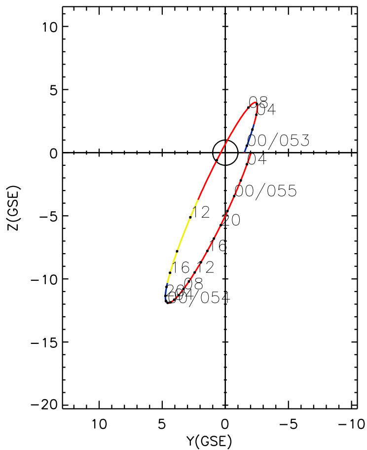
CLUSTER 2 orbit 2014 052 (02/21) 23:06 UT to 2014 055 (02/24) 05:21 UT
