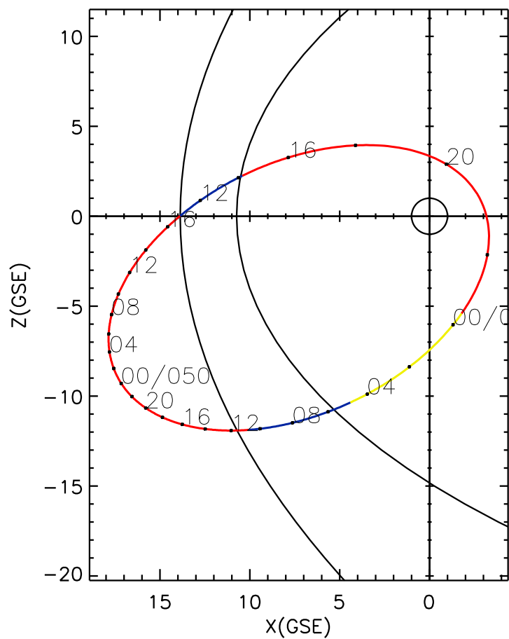
CLUSTER 2 orbit 2014 048 (02/17) 10:36 UT to 2014 050 (02/19) 16:51 UT
