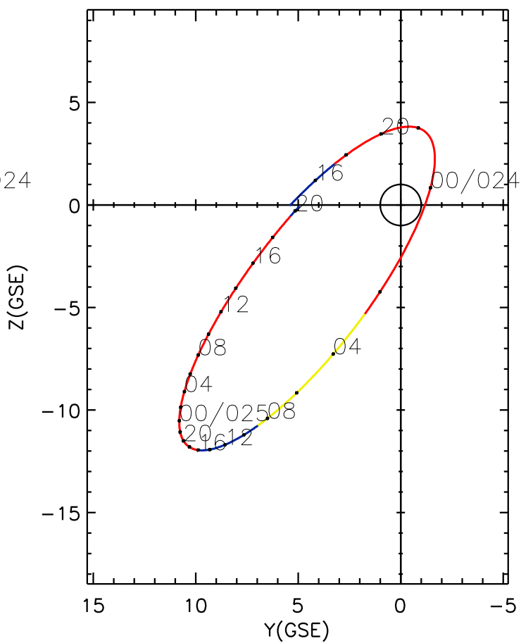
CLUSTER 2 orbit 2014 023 (01/23) 14:06 UT to 2014 025 (01/25) 20:21 UT
