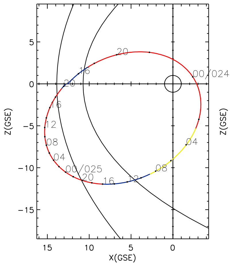
CLUSTER 2 orbit 2014 023 (01/23) 14:06 UT to 2014 025 (01/25) 20:21 UT
