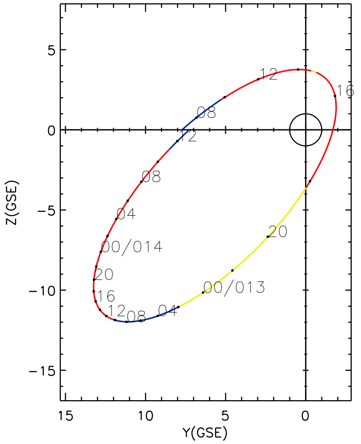
CLUSTER 2 orbit 2014 012 (01/12) 06:46 UT to 2014 014 (01/14) 13:01 UT
