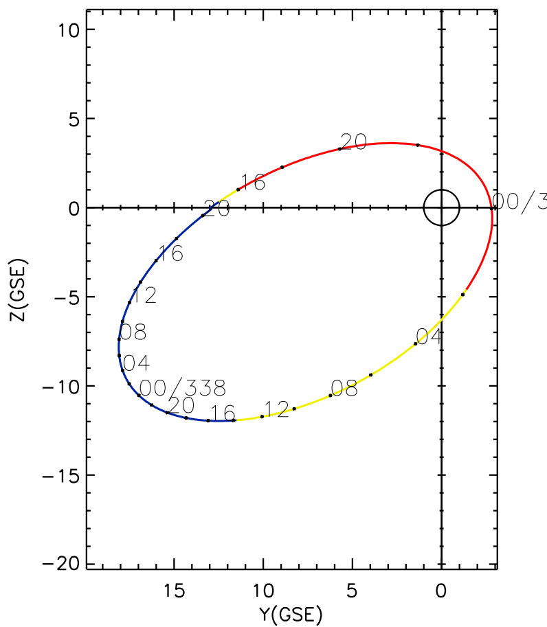
CLUSTER 2 orbit 2013 336 (12/02) 14:21 UT to 2013 338 (12/04) 20:36 UT
