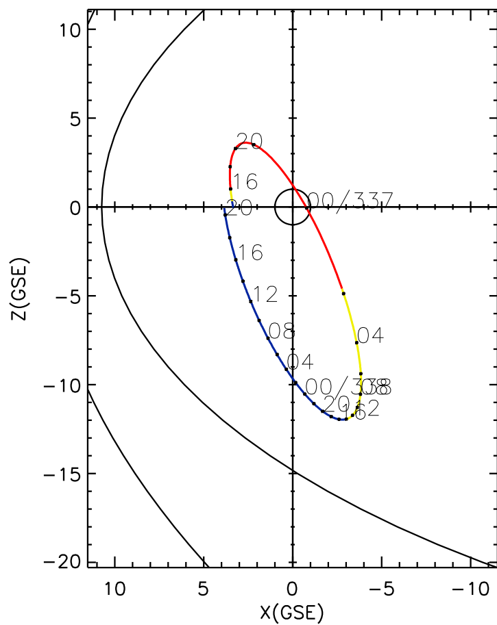
CLUSTER 2 orbit 2013 336 (12/02) 14:21 UT to 2013 338 (12/04) 20:36 UT
