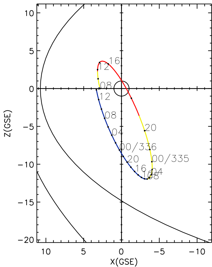
CLUSTER 2 orbit 2013 334 (11/30) 07:56 UT to 2013 336 (12/02) 14:11 UT
