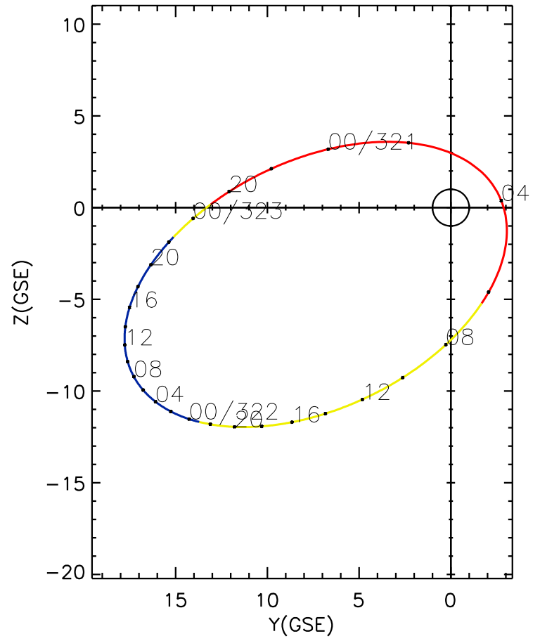
CLUSTER 2 orbit 2013 320 (11/16) 18:36 UT to 2013 323 (11/19) 00:51 UT
