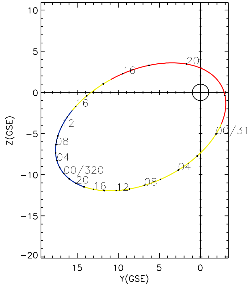
CLUSTER 2 orbit 2013 318 (11/14) 12:21 UT to 2013 320 (11/16) 18:36 UT
