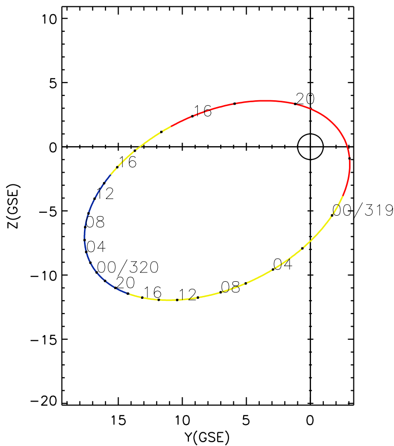
CLUSTER 2 orbit 2013 318 (11/14) 12:11 UT to 2013 320 (11/16) 18:26 UT
