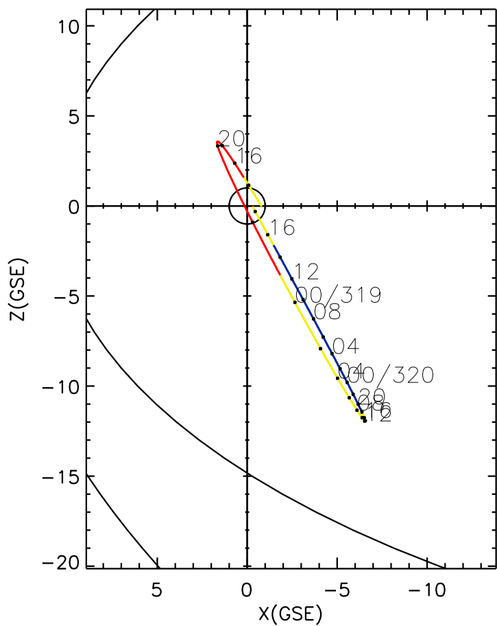
CLUSTER 2 orbit 2013 318 (11/14) 12:11 UT to 2013 320 (11/16) 18:26 UT
