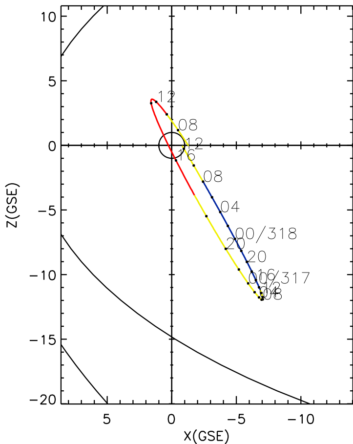
CLUSTER 2 orbit 2013 316 (11/12) 06:06 UT to 2013 318 (11/14) 12:21 UT
