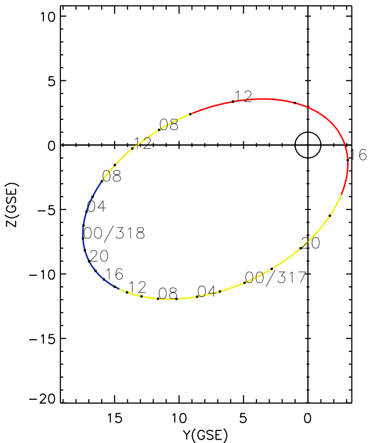
CLUSTER 2 orbit 2013 316 (11/12) 06:06 UT to 2013 318 (11/14) 12:21 UT
