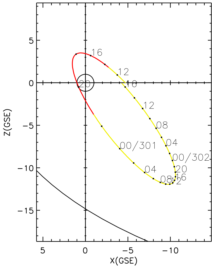
CLUSTER 2 orbit 2013 300 (10/27) 10:31 UT to 2013 302 (10/29) 16:41 UT
