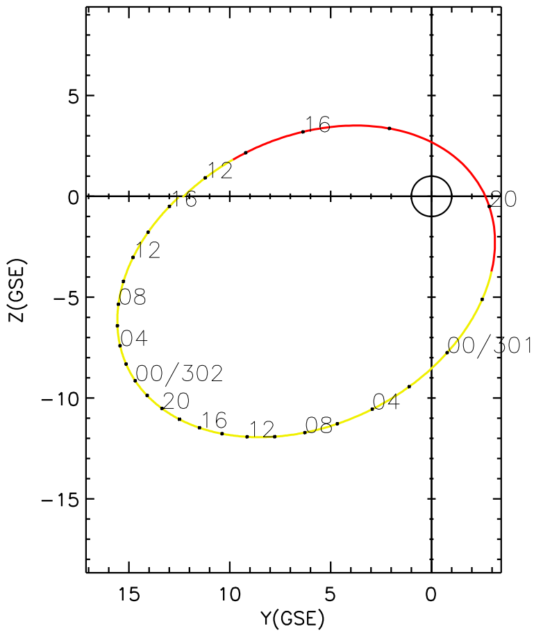
CLUSTER 2 orbit 2013 300 (10/27) 10:31 UT to 2013 302 (10/29) 16:41 UT
