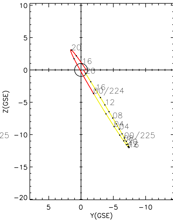
CLUSTER 2 orbit 2013 223 (08/11) 14:31 UT to 2013 225 (08/13) 20:46 UT
