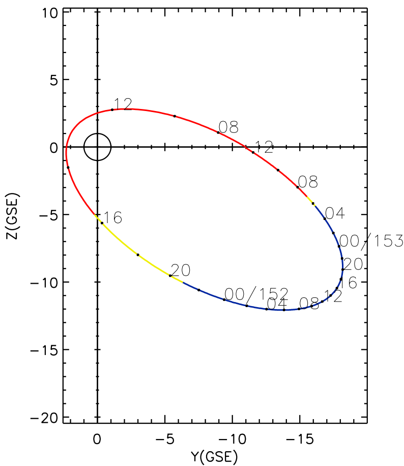
CLUSTER 2 orbit 2013 151 (05/31) 06:21 UT to 2013 153 (06/02) 12:31 UT
