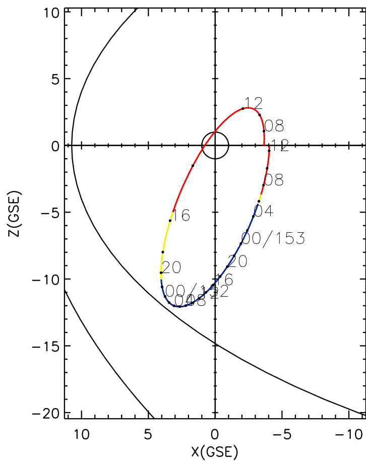
CLUSTER 2 orbit 2013 151 (05/31) 06:21 UT to 2013 153 (06/02) 12:31 UT
