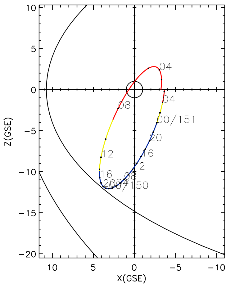
CLUSTER 2 orbit 2013 149 (05/29) 00:06 UT to 2013 151 (05/31) 06:21 UT
