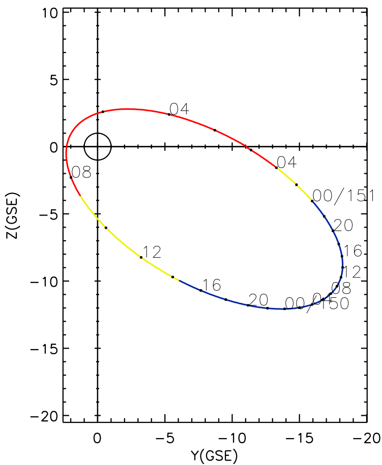
CLUSTER 2 orbit 2013 149 (05/29) 00:06 UT to 2013 151 (05/31) 06:21 UT
