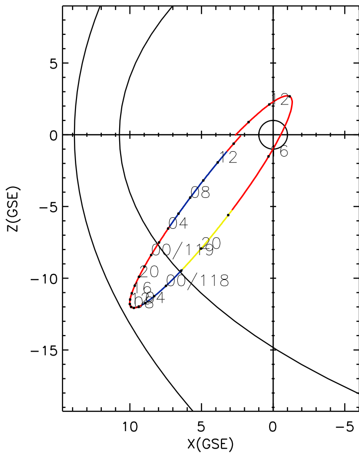
CLUSTER 2 orbit 2013 117 (04/27) 08:36 UT to 2013 119 (04/29) 14:51 UT
