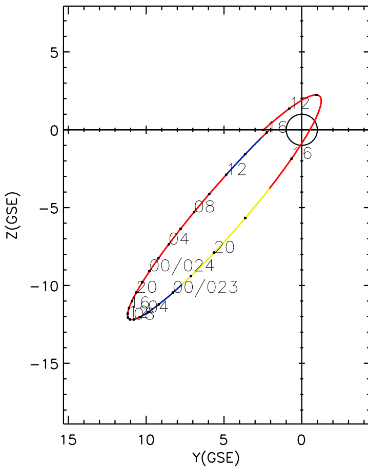
CLUSTER 2 orbit 2013 022 (01/22) 09:56 UT to 2013 024 (01/24) 16:11 UT
