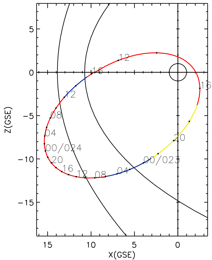
CLUSTER 2 orbit 2013 022 (01/22) 09:56 UT to 2013 024 (01/24) 16:11 UT
