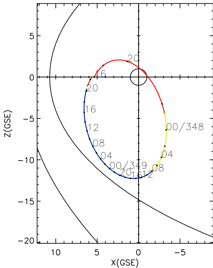
CLUSTER 2 orbit 2012 347 (12/12) 15:56 UT to 2012 349 (12/14) 22:21 UT
