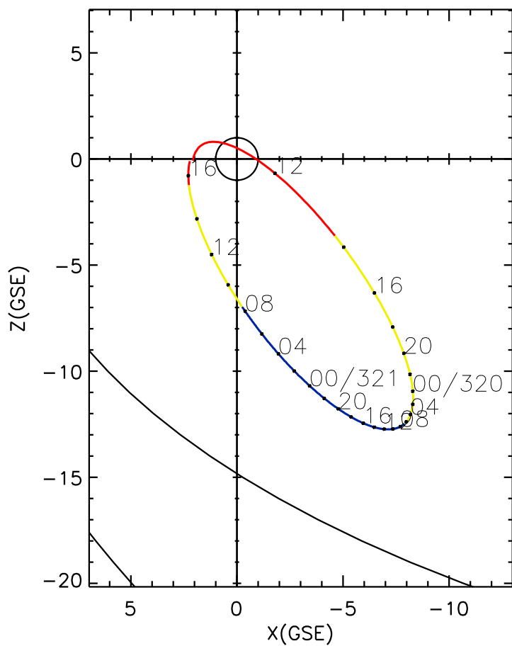
CLUSTER 2 orbit 2011 319 (11/15) 10:20 UT to 2011 321 (11/17) 16:36 UT
