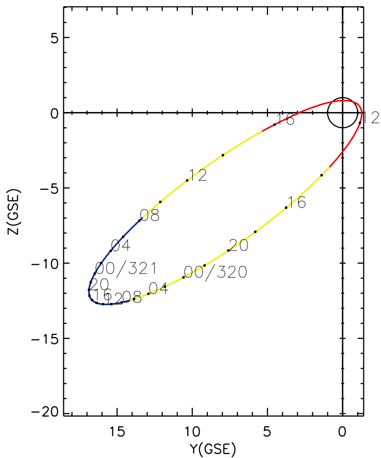
CLUSTER 2 orbit 2011 319 (11/15) 10:20 UT to 2011 321 (11/17) 16:36 UT
