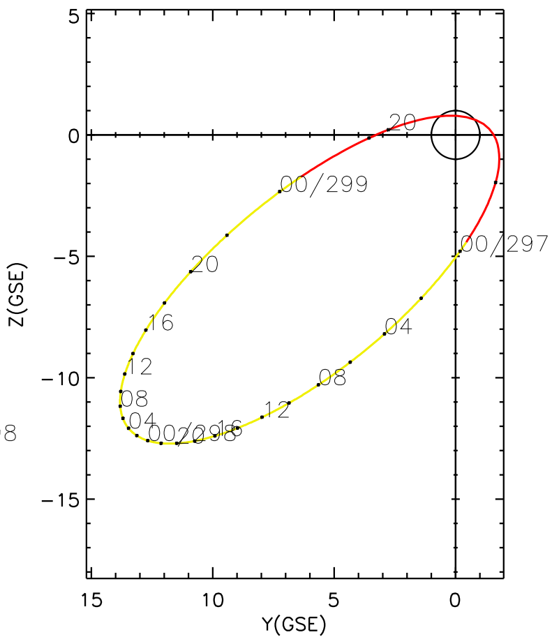
CLUSTER 2 orbit 2011 296 (10/23) 19:46 UT to 2011 299 (10/26) 02:06 UT
