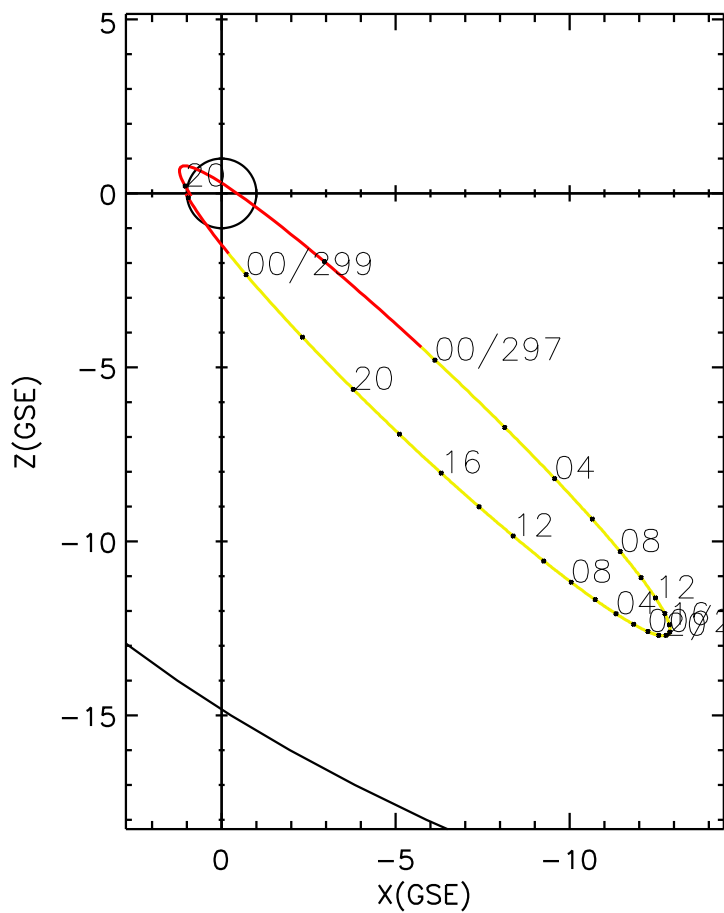
CLUSTER 2 orbit 2011 296 (10/23) 19:46 UT to 2011 299 (10/26) 02:06 UT
